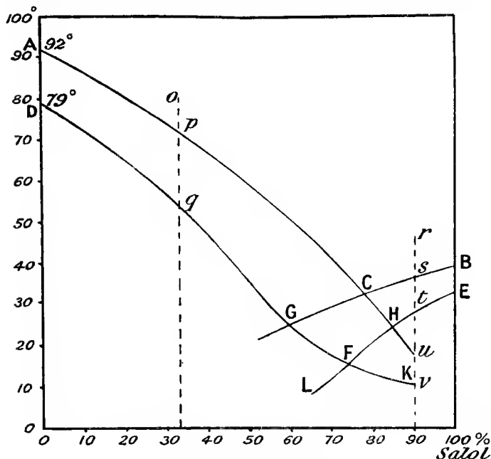
FIG. 75.—Betol and salol.
